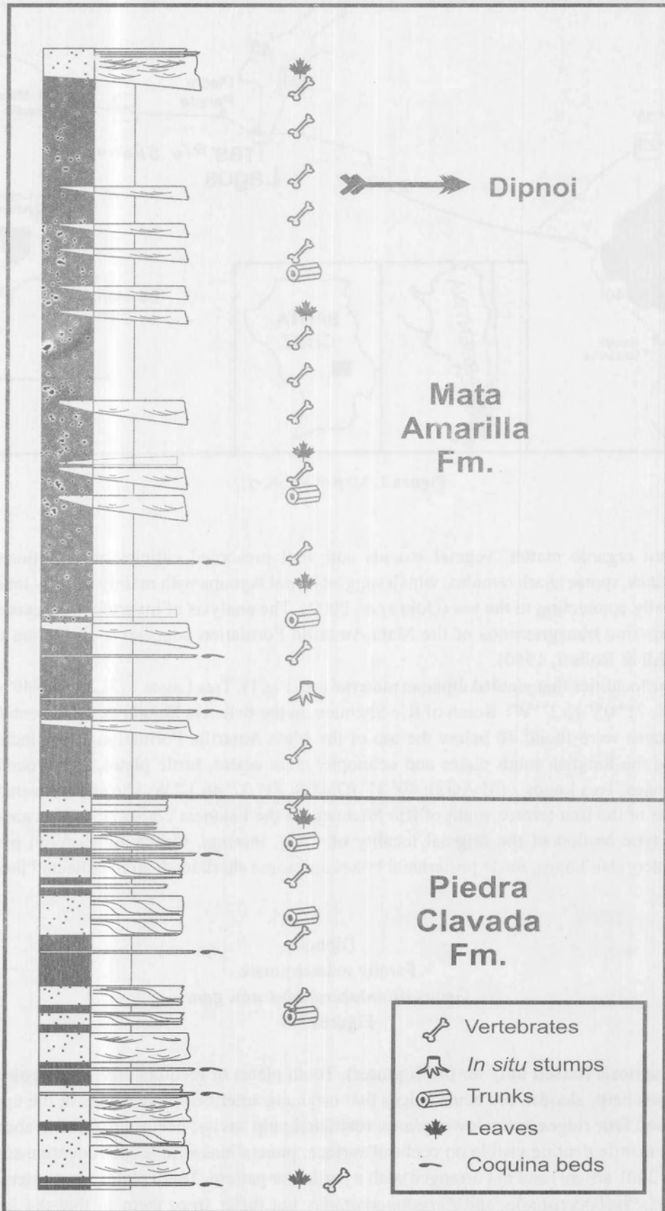
Figura 2. Stratigraphic section
